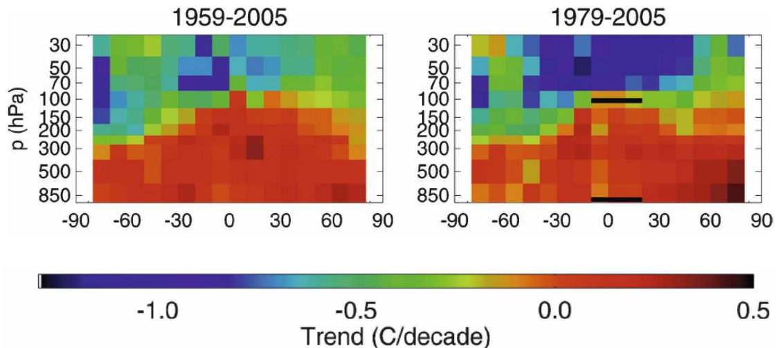
Figure 7: The warming pattern as calculated by Sherwood from the radiosonde wind data as well as the temperature data shown in Figure 1. From Fig. 6 of Sherwood 2008, camels.metoffice.gov.uk/quarc/Sherwood08_JClimate.pdf . It appears he “found” the hotspot, but look at the scale closely!
