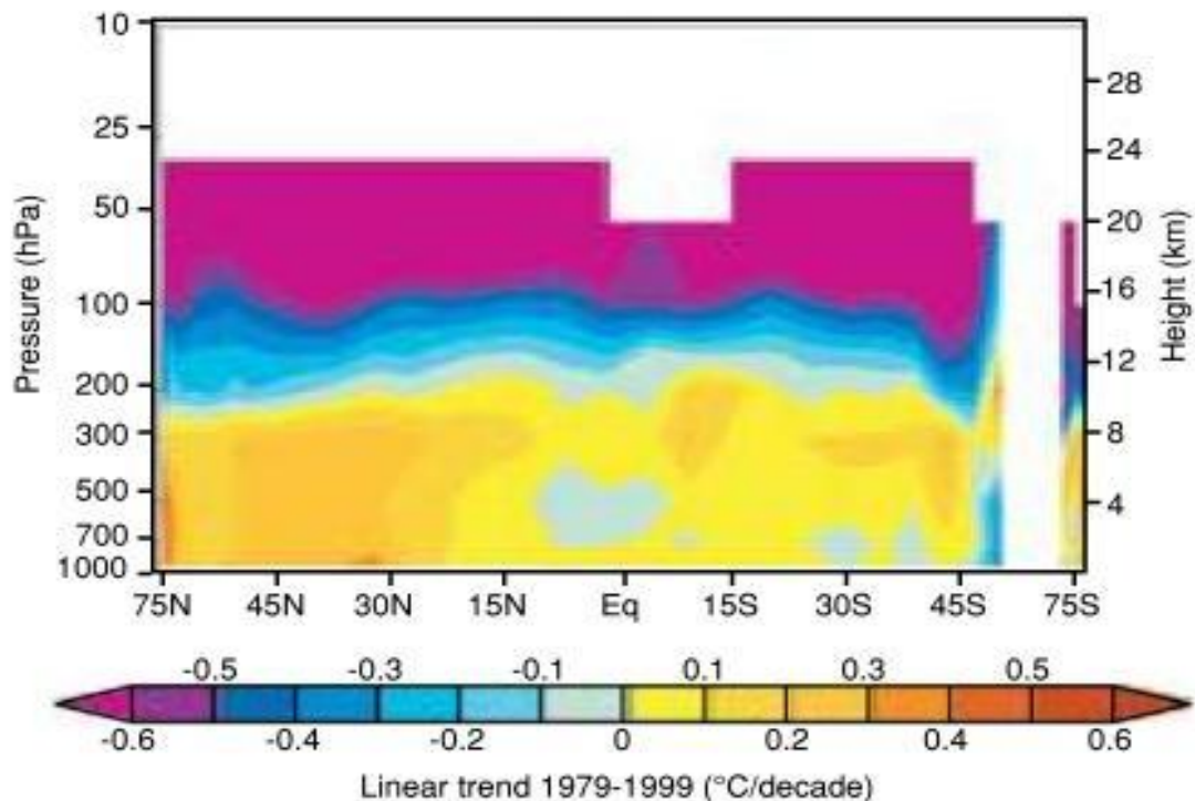
Figure 1: The observed pattern of atmospheric warming, 1979 – 1999, as per the US CCSP of 2006, part E of Figure 5.7 in section 5.5 on page 116. (Axes deblurred.)
