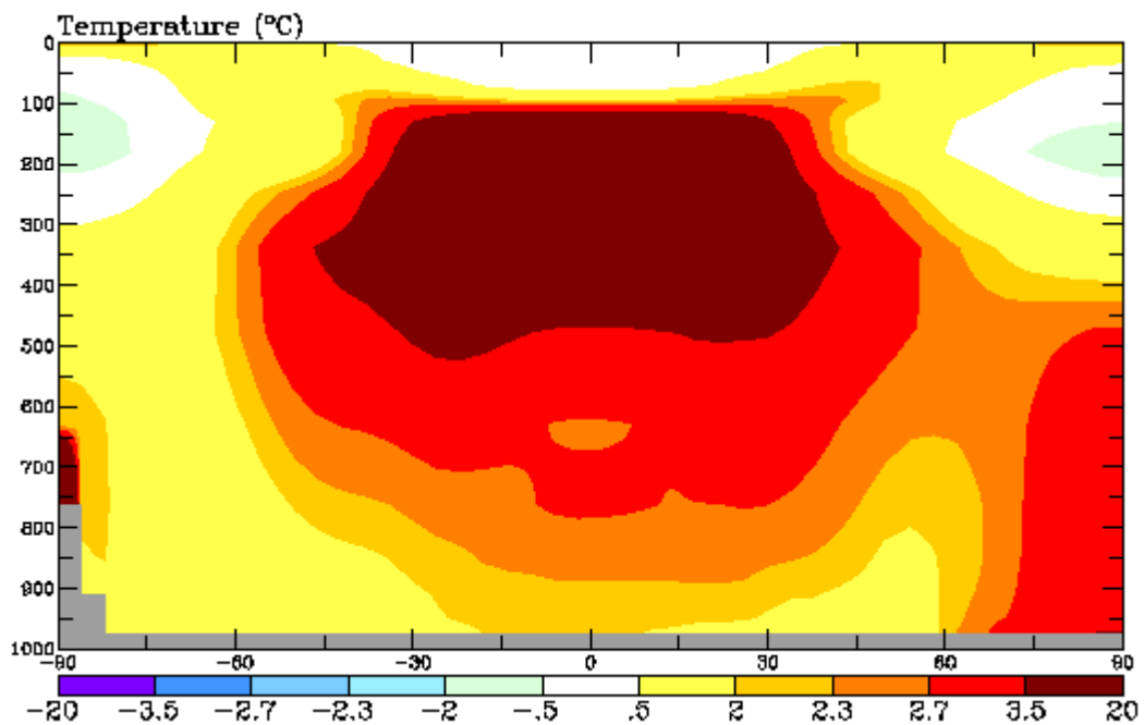
Figure 9: Signatures of a doubling of CO 2 (top) and a 2% increase in radiation from the sun (bottom), according to the GISS model. Each is dominated by a hotspot.
