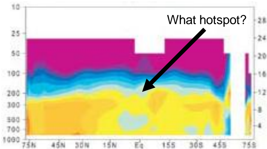
Figure 8: The observed warming pattern. If the hotspot is there, where is it?
