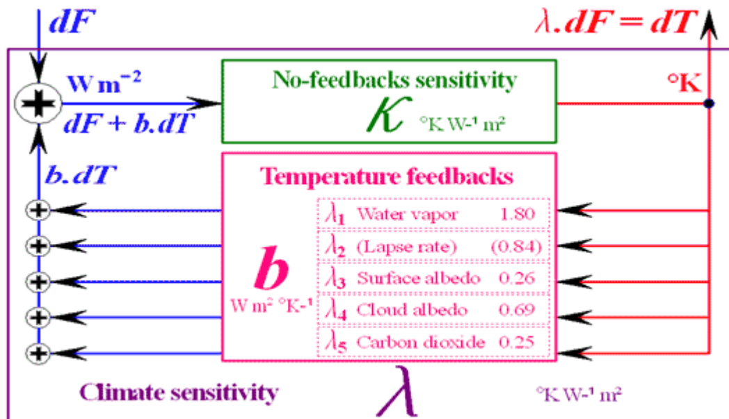
Figure 10: A perturbation dF in the incoming solar radiation (or “forcing”) is input to the earth’s climate system (purple box). It is multiplied by \kappa by the no-feedbacks climate system (green box), to produce an initial temperature perturbation dT . But dT also causes temperature feedbacks (red box) which add a further b dT to the input of the no-feedbacks climate system! After sorting out the simultaneous effects, the final temperature perturbation due to dF is dT = \kappa dF / (1 - b\kappa) .
